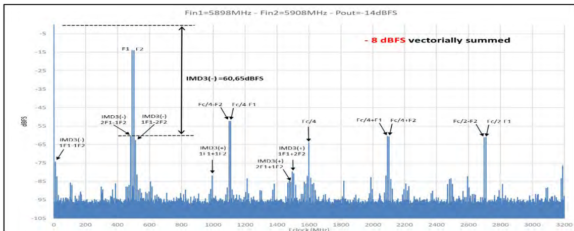
Figure 82: IMD3 – Analog Input frequency 5900 MHz – P_{out} = -14 \text{ dBFS}
