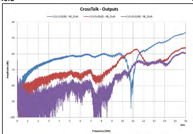
Figure 51: Cross-talk between serial outputs
