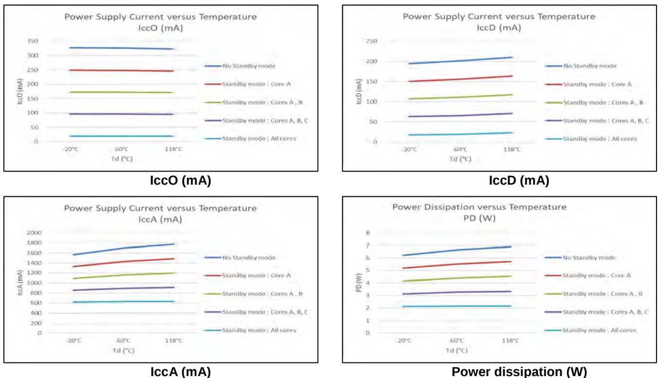
Figure 46: Current consumption and power dissipation versus temperature and standby mode
