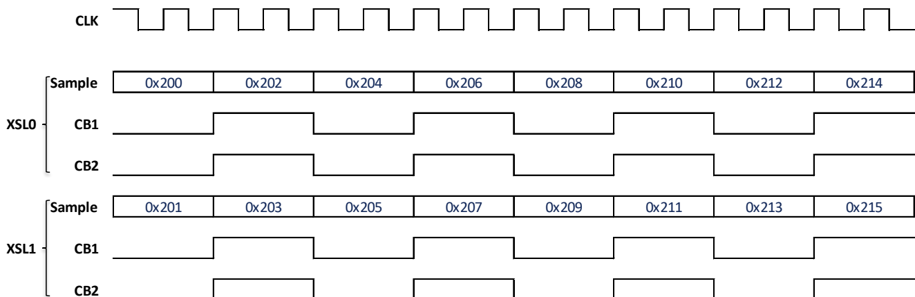
Figure 27: Chronogram of the Ramp test mode
