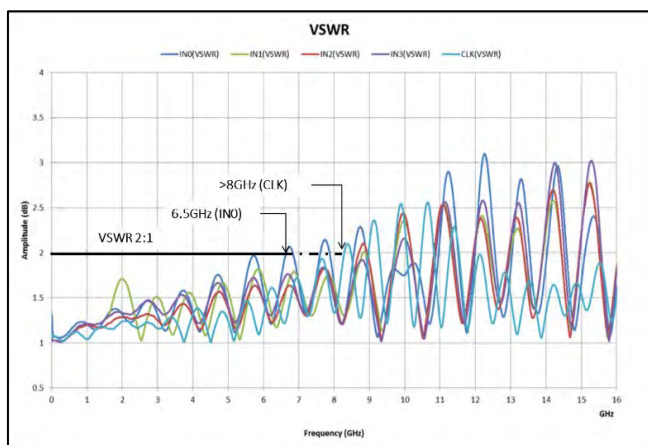
Figure 52: VSWR on analog inputs and clock
