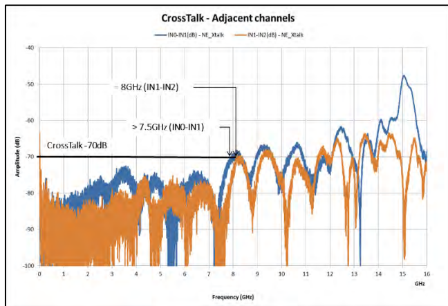
Figure 49: Cross-talk between analog input channels
