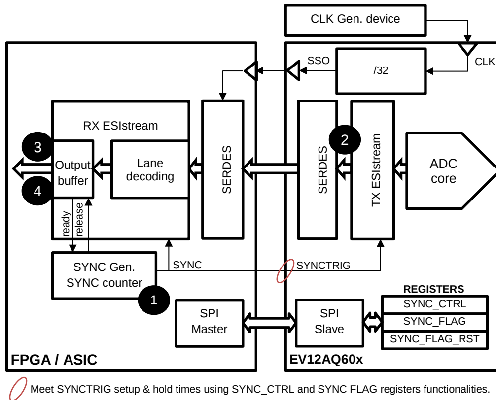
Figure 40: Deterministic latency architecture ; using SSO
