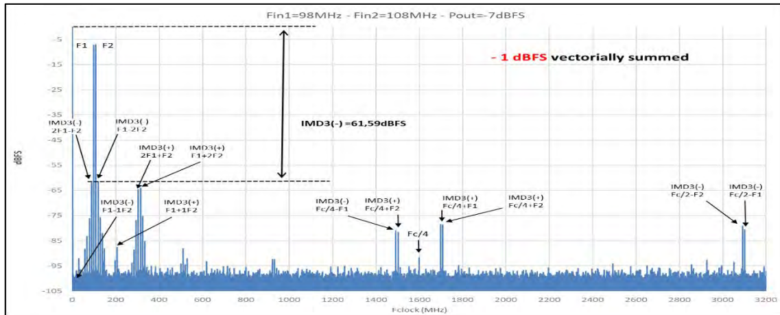
Figure 80: IMD3 – Analog Input frequency 100 MHz – P_{out} = -7 \text{ dBFS}
