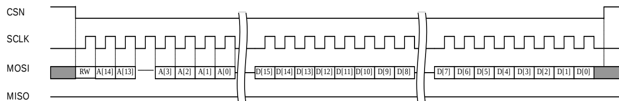
Figure 13: SPI writing
