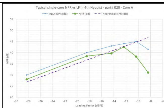
Figure 86: 4 th Nyquist NPR versus loading factor. Fs = 1.6 GSps.
