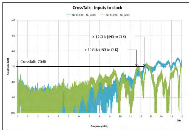
Figure 50: Cross-talk between analog inputs and clock
