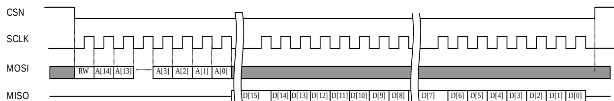
Figure 14: SPI reading
