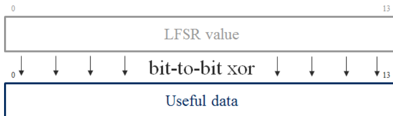
Figure 37: LFSR operation
