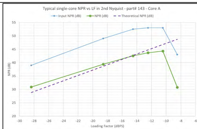
Figure 84: 2 nd Nyquist NPR versus loading factor. Fs = 1.6 GSps.
