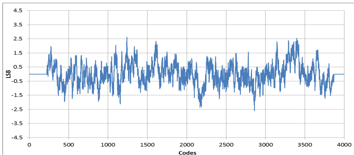
Figure 54: INL - 4-channel mode – 1.6 GSps
