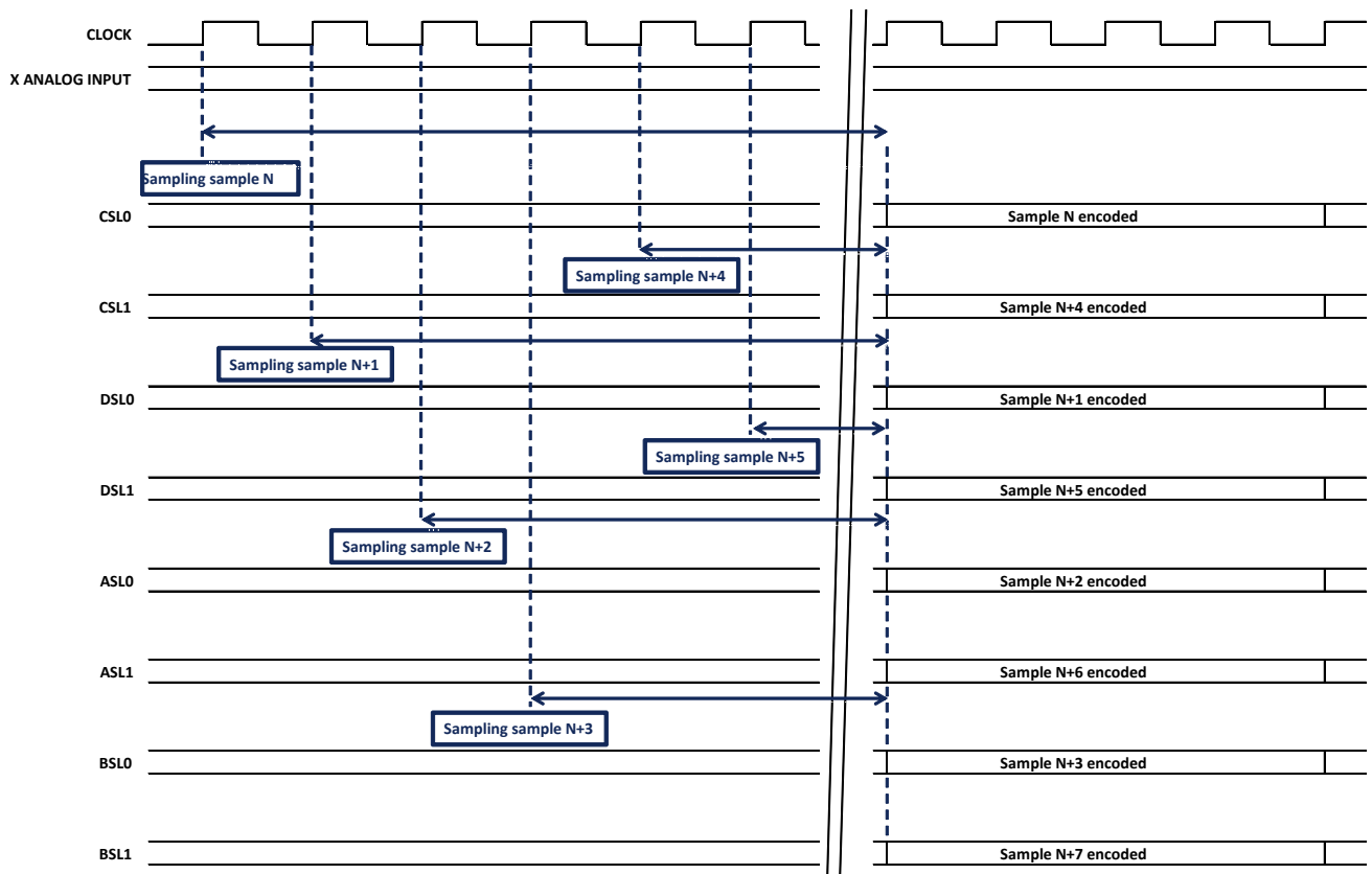
Figure 23: Timing diagram in serial interface in 1-channel mode
