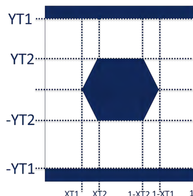
Figure 3 Serial link eye diagram
