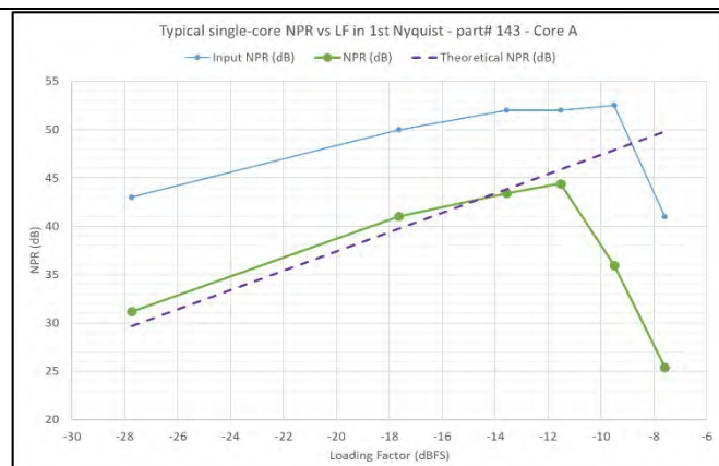
Figure 83: 1 st Nyquist NPR versus loading factor. Fs = 1.6 GSps.
