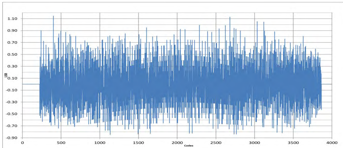
Figure 57: DNL - 4-channel mode – 1.6 GSps
