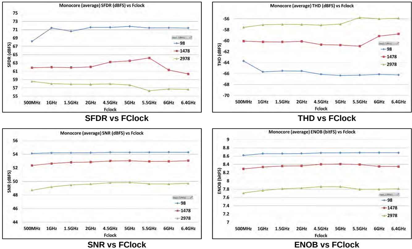
Figure 69: Performance vs Fclock - 4-channel mode – 1.6 GSps
