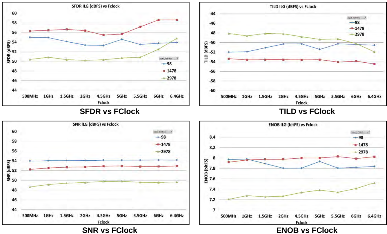
Figure 70: Performance vs Fclock - 1-channel mode – 6.4 GSps
