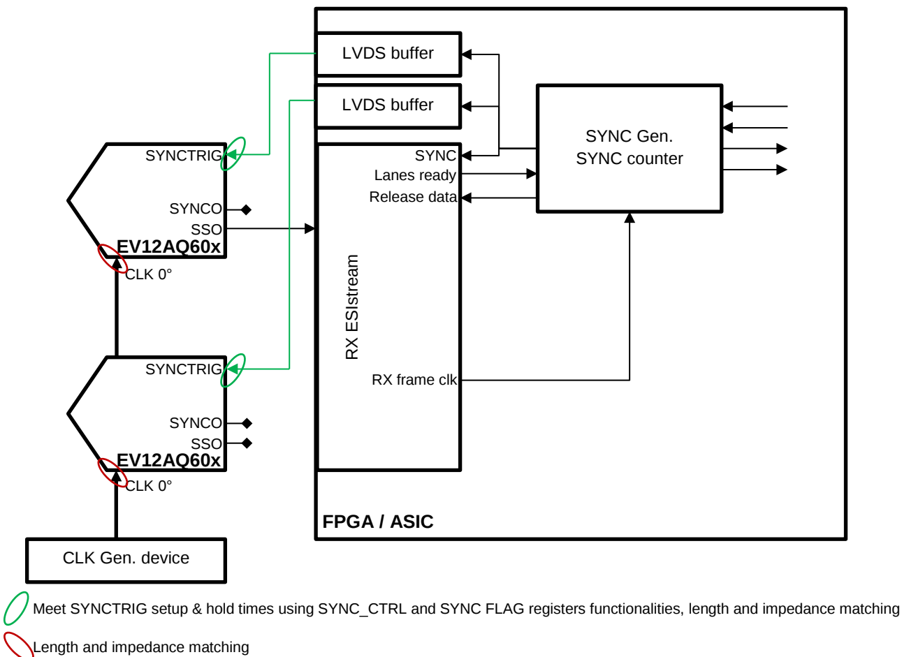
Figure 44: Multi-devices synchronization deterministic system ; using sync point-to-point
