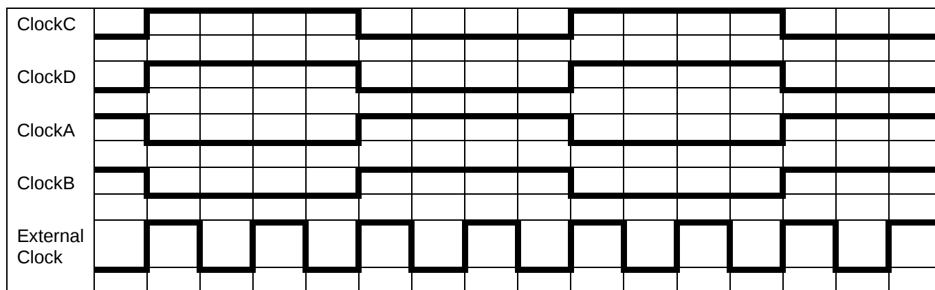
Figure 20: Clocks for two cores interleaving - configuration 2: Interleaving of A and C and interleaving of B and D CLK_MODE_SEL = 2
