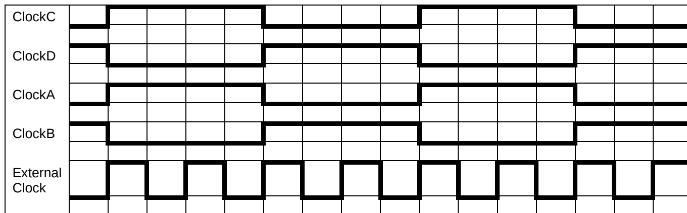
Figure 19: Clocks for two cores interleaving - configuration 1: Interleaved of A and B and interleaved of C and D CLK_MODE_SEL = 1
