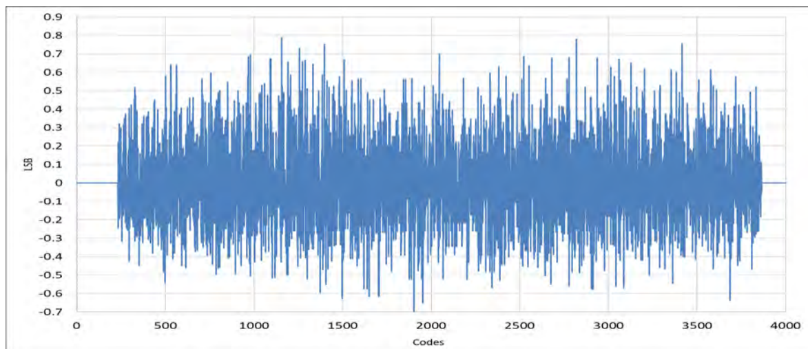
Figure 58: DNL - 2-channel mode – 3.2 GSps
