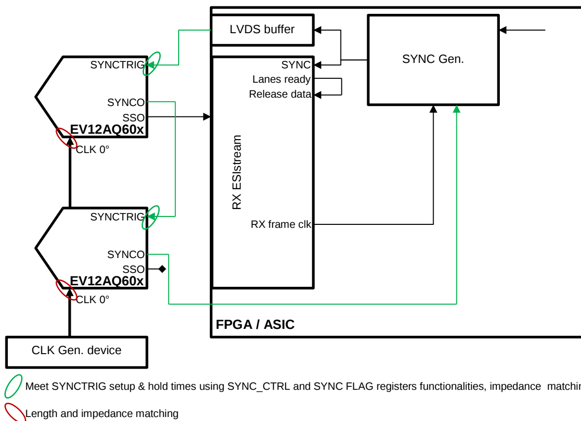
Figure 42: Multi-devices synchronization ; using sync chaining
