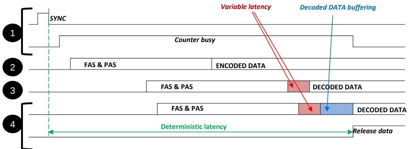
Figure 41: Deterministic latency time chart
