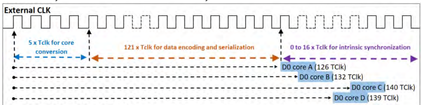
Figure 5: Latency example 1
