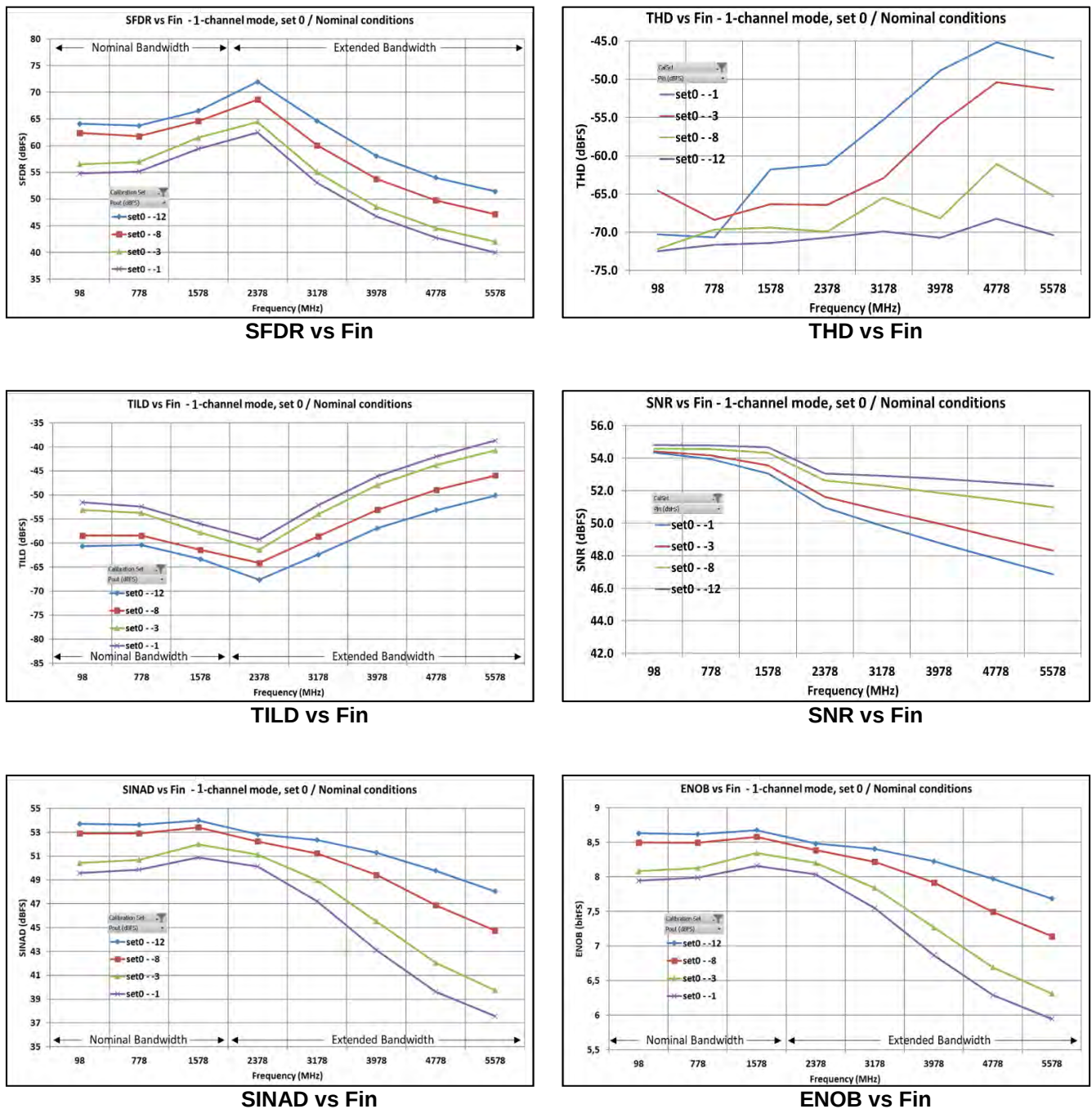
Figure 63: Performance vs Analog input frequencies - 1-channel mode – 6.4 GSps - Calibration set: CalSet0 -
