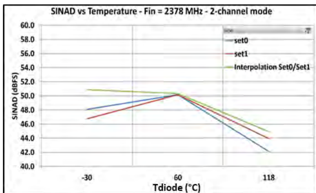
SINAD vs temperature
