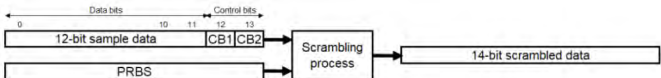
Figure 33: 14-bit scrambled frame
