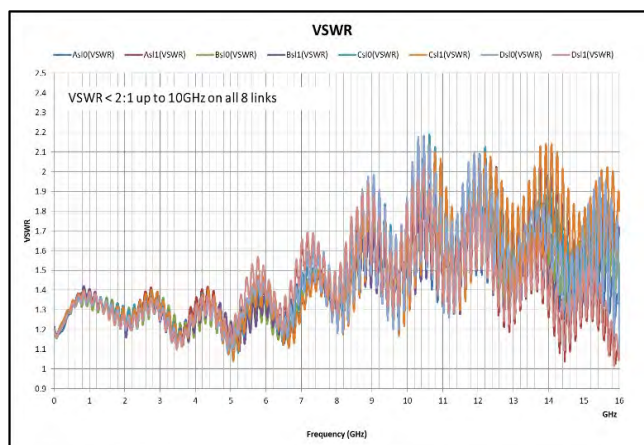
Figure 53: VSWR on serial output
