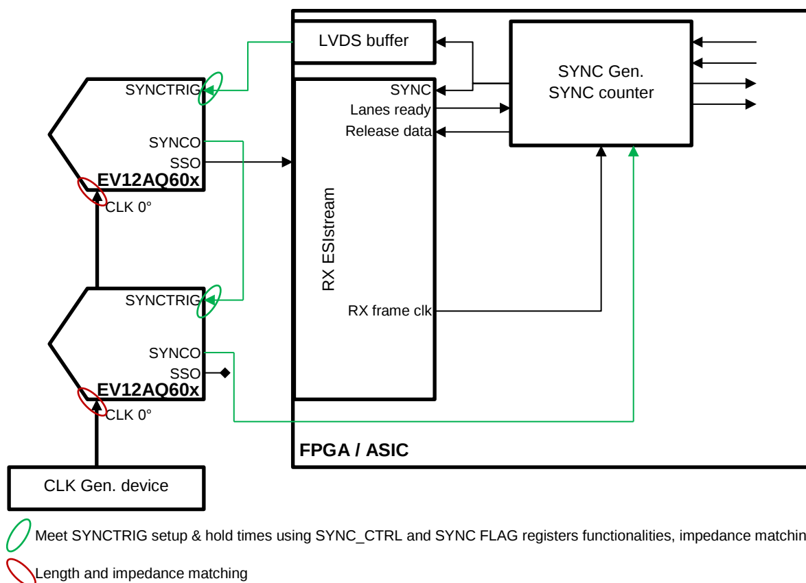
Figure 43: Multi-devices synchronization deterministic system ; using sync chaining
