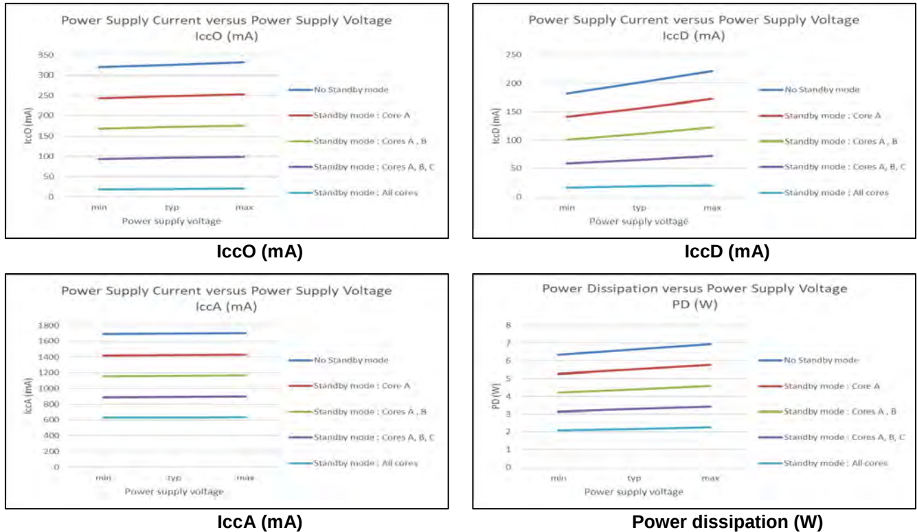
Figure 45: Current consumption and power dissipation versus supply voltage and standby mode
