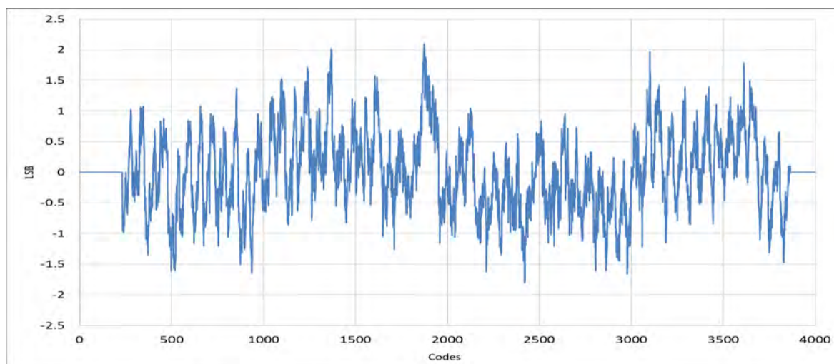
Figure 55: INL - 2-channel mode – 3.2 GSps
