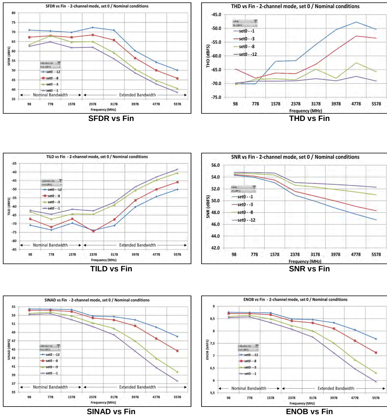
Figure 61: Performance vs Analog input frequencies - 2-channel mode – 3.2 GSps - Calibration set: CalSet0 -
