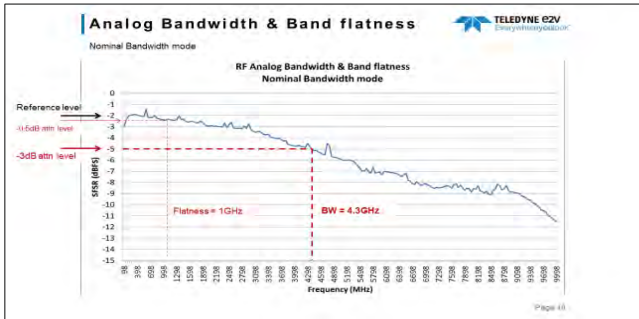
Figure 47: Nominal Bandwidth
