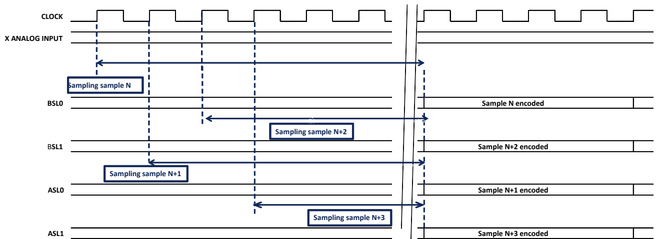
Figure 24: Timing diagram in serial interface in 2-channel mode
