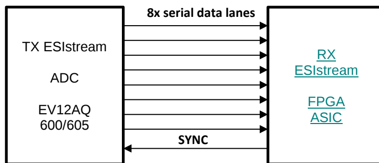
Figure 32: ESIsstream system example using EV12AQ60x ADC
