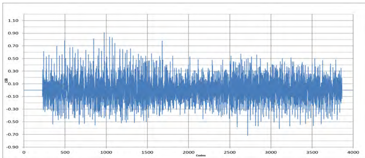
Figure 59: DNL - 1-channel mode – 6.4 GSps
