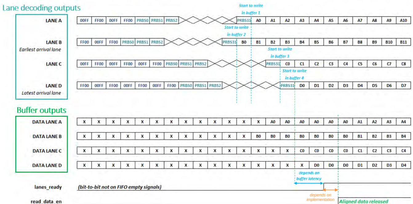
Figure 39: Multi-lanes synchronization time chart ; using FIFO as output buffer
