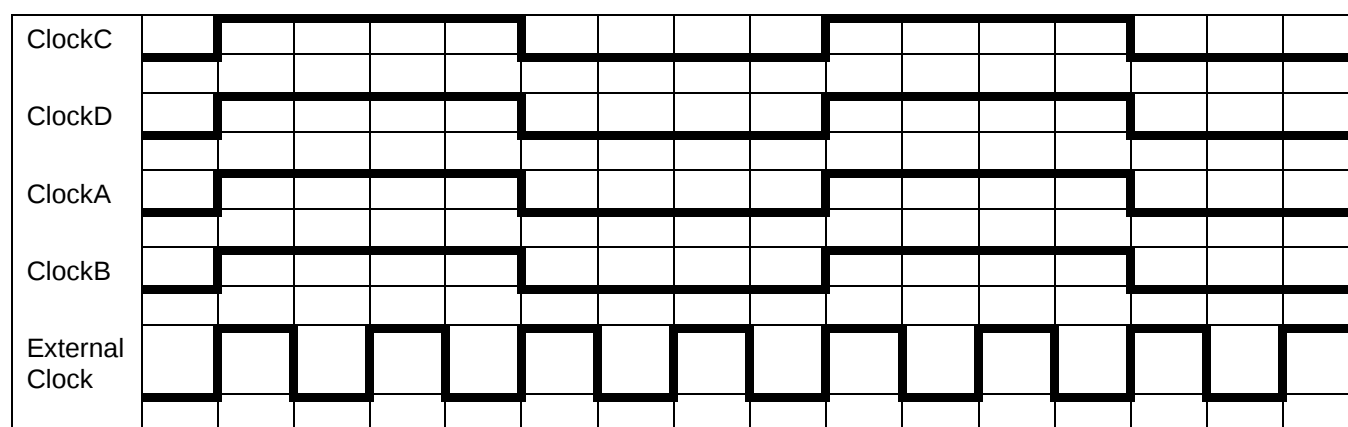
Figure 18: Clocks for four cores aligned averaging or four channels, CLK_MODE_SEL = 3
