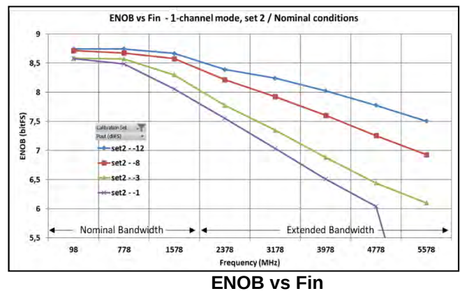
Figure 64: Performance vs Analog input frequencies - 1-channel mode – 6.4 GSps - Calibration set: CalSet2 -
