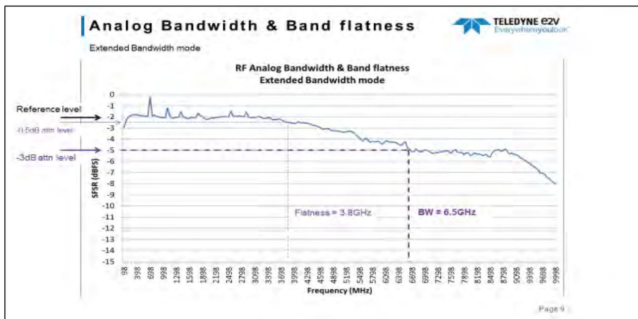
Figure 48: Extended Bandwidth
