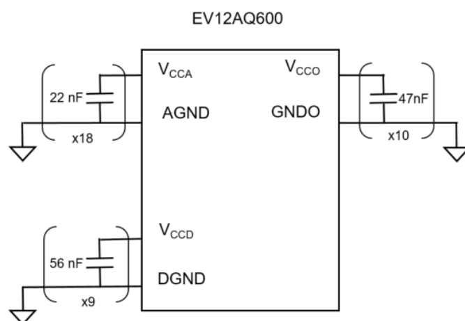
Figure 31: Power Supplies decoupling scheme
