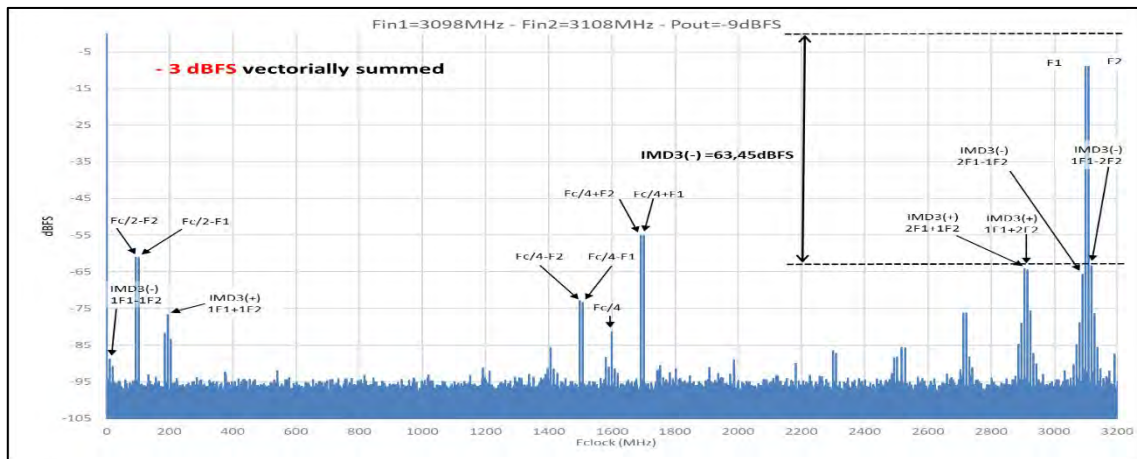
Figure 81: IMD3 – Analog Input frequency 3100 MHz – P_{out} = -9 \text{ dBFS}
