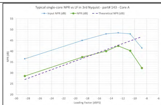
Figure 85: 3 rd Nyquist NPR versus loading factor. Fs = 1.6 GSps.
