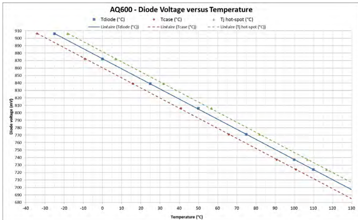
Figure 30: Voltage vs temperature.
