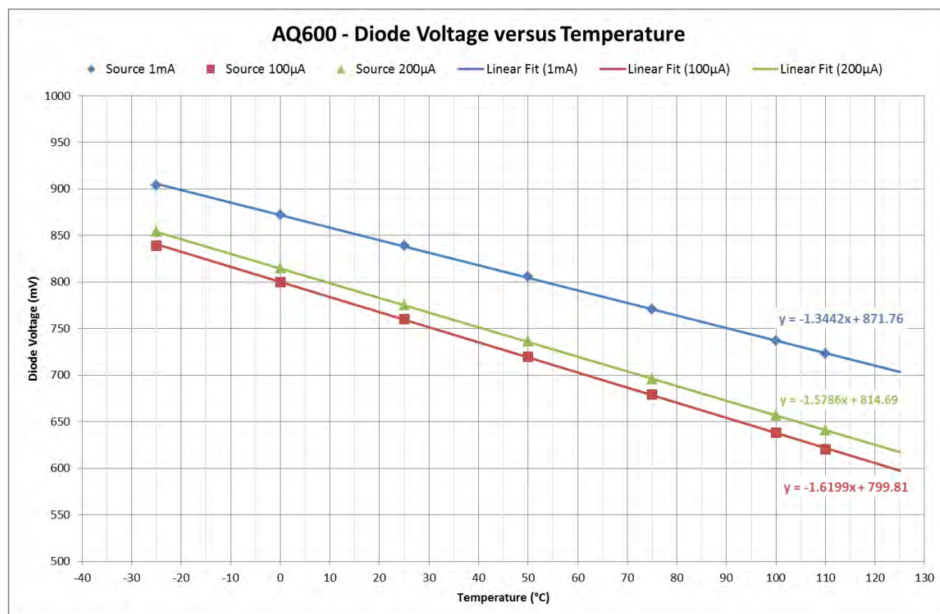
Figure 29: Diode voltage vs temperature for 3 different input currents (blue: 1 mA, green: 200 µA, red: 100 µA)
