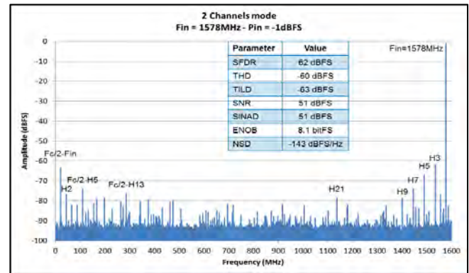
2-channel mode – 3.2 GSps – Fin = 1578 MHz
