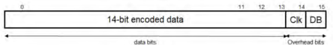
Figure 38: Frame format after encoding
