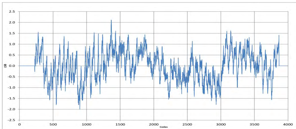
Figure 56: INL - 1-channel mode – 6.4 GSps
