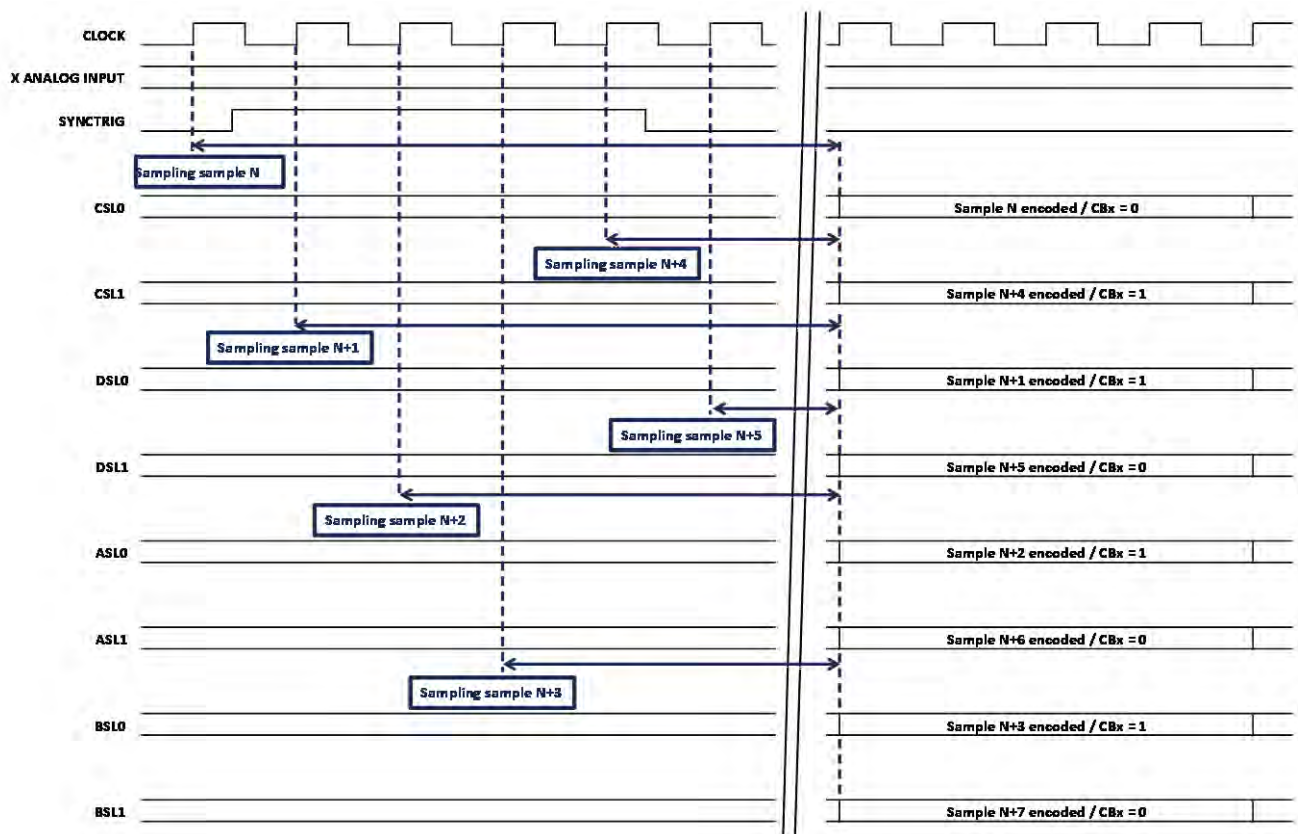
Figure 22: Trigger mode timing diagram in serial interface
