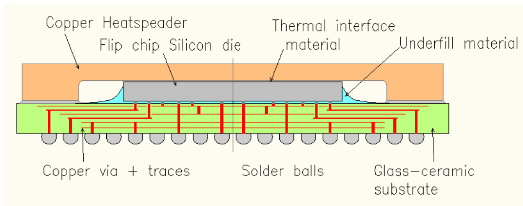
Figure 7: Package cross-section
